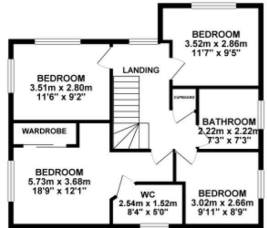
1ST FLOOR 61.15 sq. m. ( 658.16 sq. ft. )
